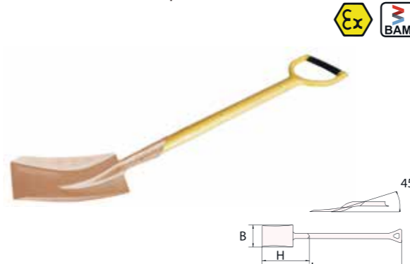
防爆装柄方锹 Shovel, Square
