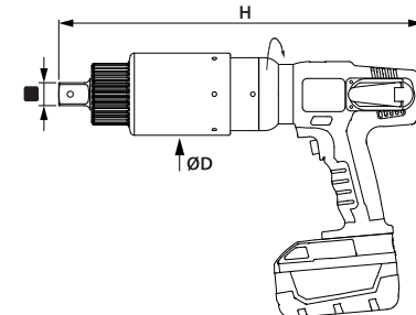
LDA series – straight version
